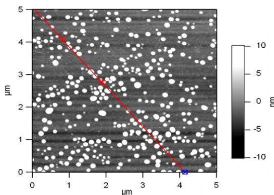
Figure 2. Atomic force microscopy (AFM) image of NP1 indicates that the nanoparticles are uniformly spherical and between 30 and 50 nm in diameter.
