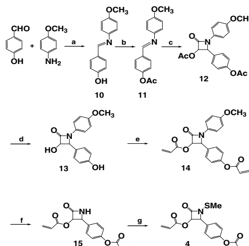
Scheme 4. Reagents and conditions: (a) CSA, CH 2 Cl 2 , rt; (b) acetyl chloride, Et 3 N, CH 2 Cl 2 , 92% overall; (c) acetoxyacetyl chloride, Et 3 N, CH 2 Cl 2 , 65%; (d) KOH, MeOH, acetone, 0 °C, 92%; (e) acryloyl chloride, Et 3 N, CH 2 Cl 2 , 93%; (f) ceric ammonium nitrate, CH 3 CN, H 2 O, 0 °C, 84%; (g) N -methylthiophthalimide, Hunig's base, CH 2 Cl 2 , reflux, 72%.
