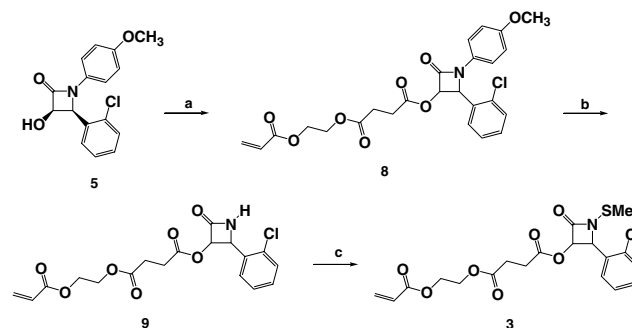
Scheme 3. Reagents and conditions: (a) mono-2-acryloyloxyethyl succinate, EDCI, DMAP, CH 2 Cl 2 , rt, 77%; (b) ceric ammonium nitrate, H 2 O, CH 3 CN, 0 °C, 86%; (c) N -methylthiophthalimide, CH 2 Cl 2 , Hunig's base, reflux, 72%.
