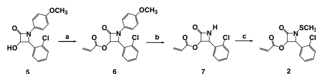
Scheme 2. Reagents and conditions: (a) acryloyl chloride, NaH, CH 2 Cl 2 , 85%; (b) ceric ammonium nitrate, CH 3 CN, H 2 O, 0 °C, 90%; (c) N -methylthiophthalimide, CH 2 Cl 2 , Hunig's base, reflux, 82%.
