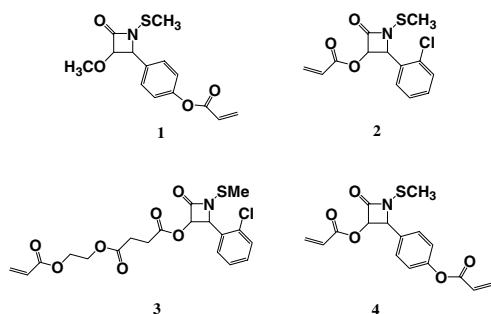
Figure 1. N -Thiolated β-lactam acrylate monomers 1–4.
